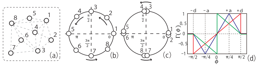
Fig. 1. (a) Sensor networks of N nodes ( N = 8 , for instance). (b), (c) Resulting timing allocation for type1 and type2 functions, and (d) Function \Gamma with a tuning parameter a (blue line); type1 function (green line, a = 0 ), type2 function (red line, a = d )
