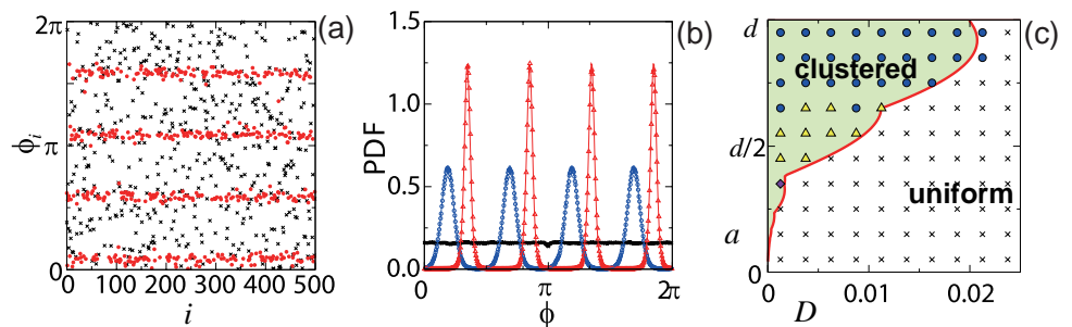
Fig. 2. (a) Typical snapshot of phase variables \phi_i from Eq.(1) for the type1 and type2 functions. (b) Normalized histograms and PDFs of \phi . Data points and curves are respectively obtained from Eq. (1) and Eq. (3), showing a good match. (c) Stability diagram of the uniform state and observed patterns.
